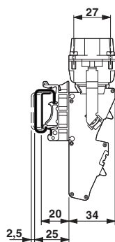
Dimensioned drawing
