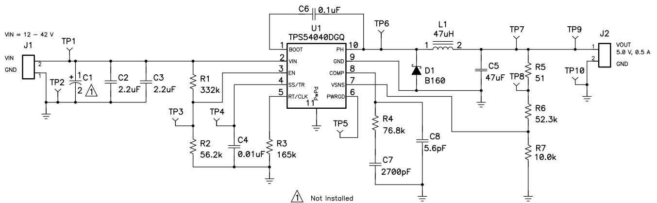
Figure 14. TPS54040EVM-456 Schematic
