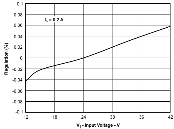
Figure 4. TPS54040EVM-456 Line Regulation
