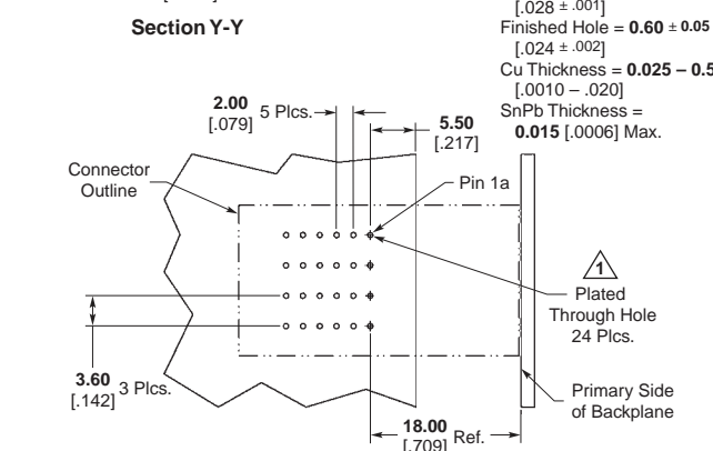
Recommended PCB Hole Layout
