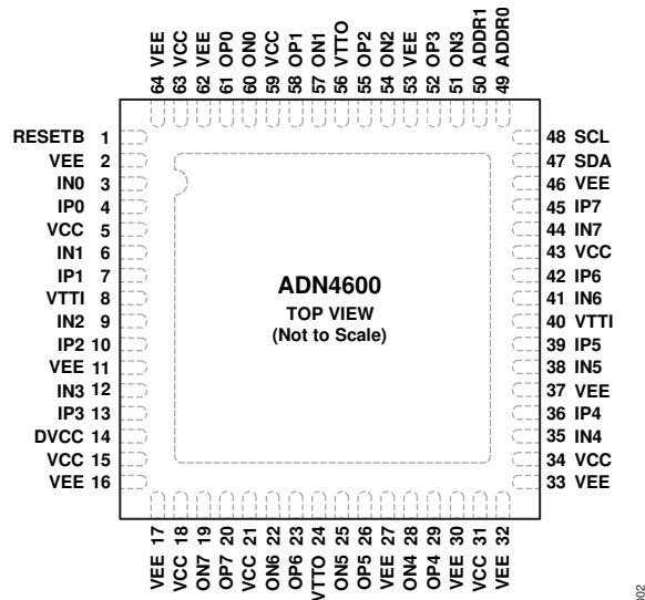
Figure 3. Pin Configuration
