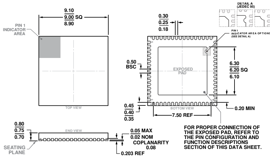
Figure 33. 64-Lead Lead Frame Chip Scale Package [LFCS] 9 mm × 9 mm Body and 0.75 mm Package Height (CP-64-17) Dimensions shown in millimeters
