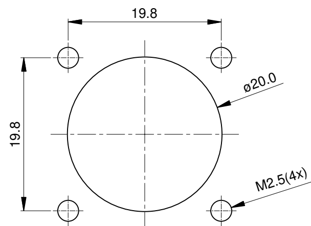
MOUNTING HOLE
