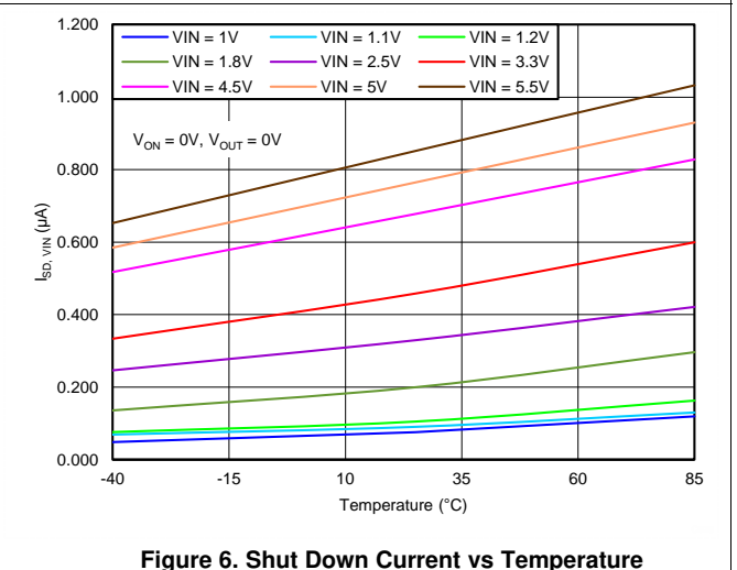
Figure 6. Shut Down Current vs Temperature
