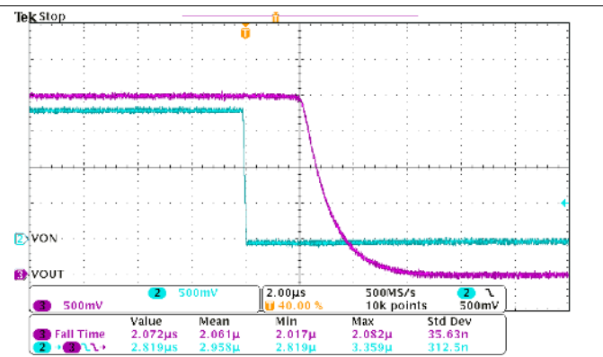
Figure 25. Turn-Off Response Time ( V_{IN} = 3.3\text{ V} , C_{IN} = 1\ \mu\text{F} , C_{OUT} = 0.1\ \mu\text{F} , R_{OUT} = 10\ \Omega )
