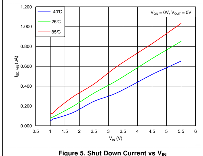
Figure 5. Shut Down Current vs V_{IN}
