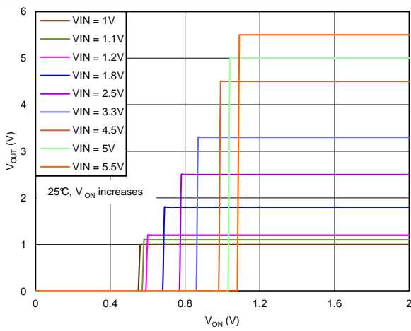
Figure 9. Output Voltage vs V ON Rising
