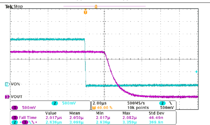
Figure 27. Turn-Off Response Time ( V_{IN} = 2.5\text{ V} , C_{IN} = 1\ \mu\text{F} , C_{OUT} = 0.1\ \mu\text{F} , R_{OUT} = 10\ \Omega )
