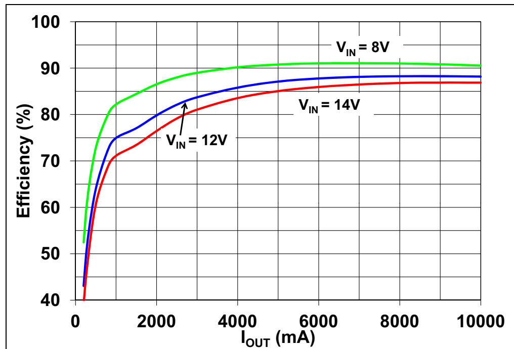
FIGURE C-1: Efficiency.
