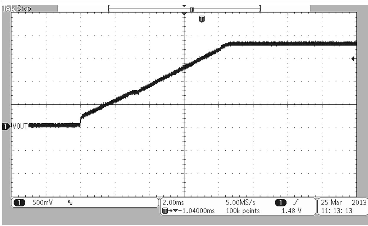
FIGURE C-14: Soft Start.
