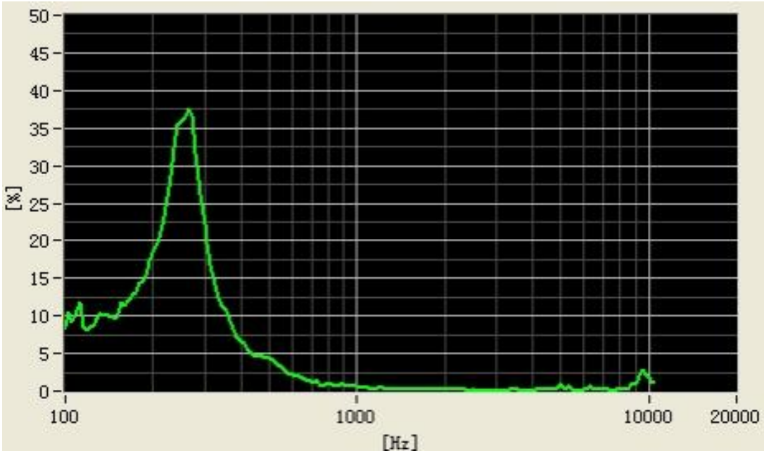
1.4 Total Harmonic Distortion Curve (at sine wave 3v,0.1m,using SOUNDCHECK testing)
