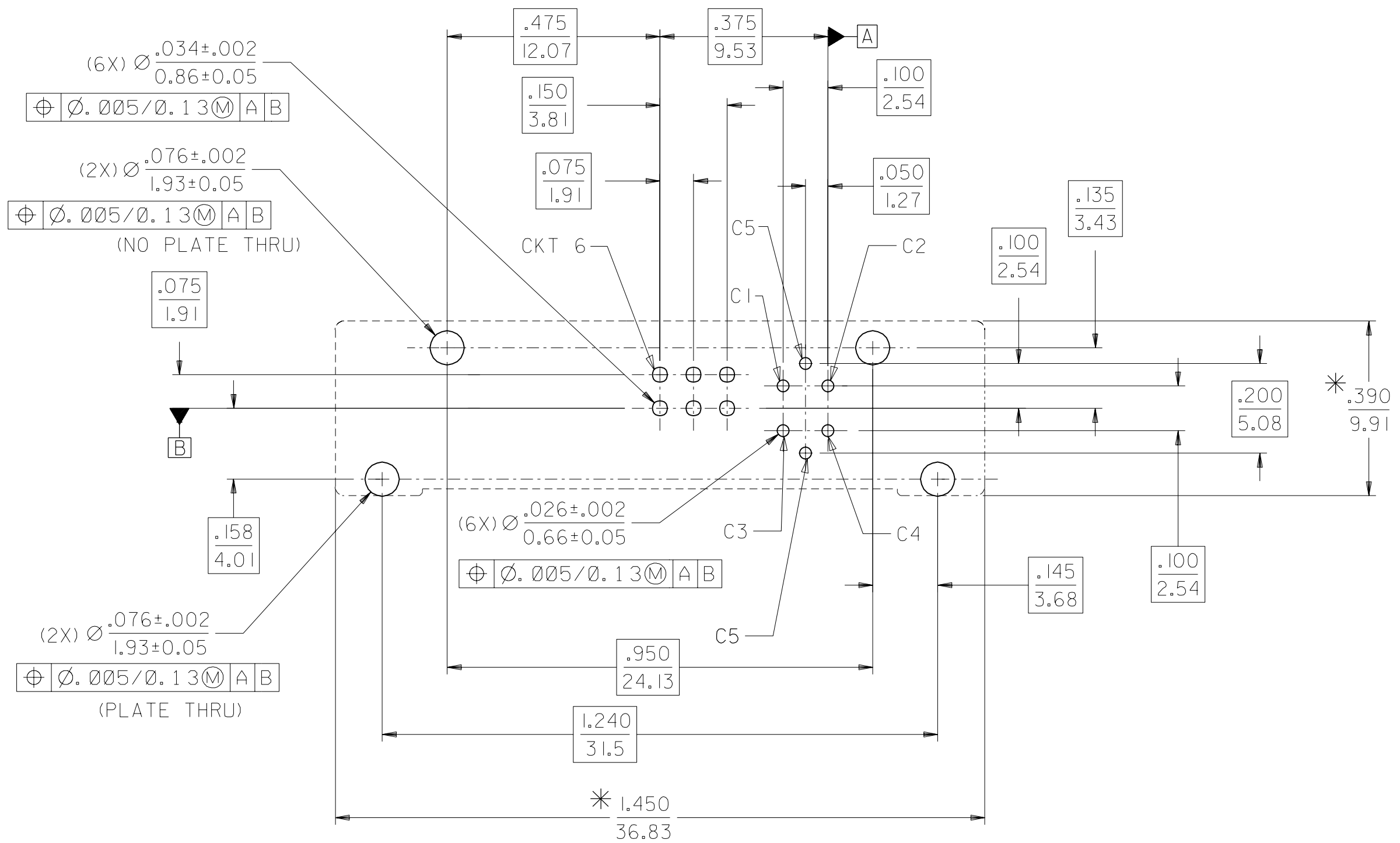
RECOMMENDED PCB LAYOUT
