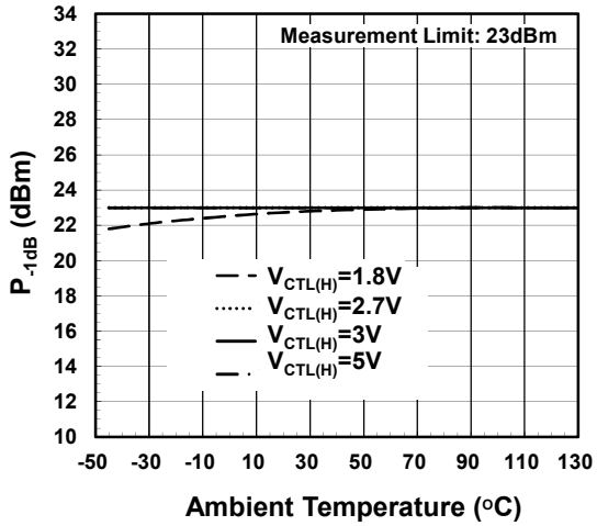
P -1dB vs Temperature (f=8.5GHz, V CTL(L) =0V, PC-P1 ON)
