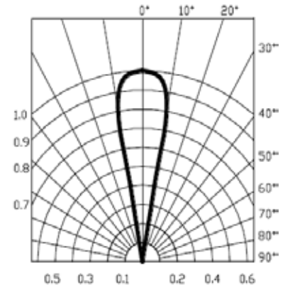
Radiation Diagram
