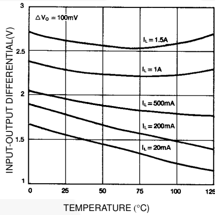
Figure 4. Dropout Voltage
