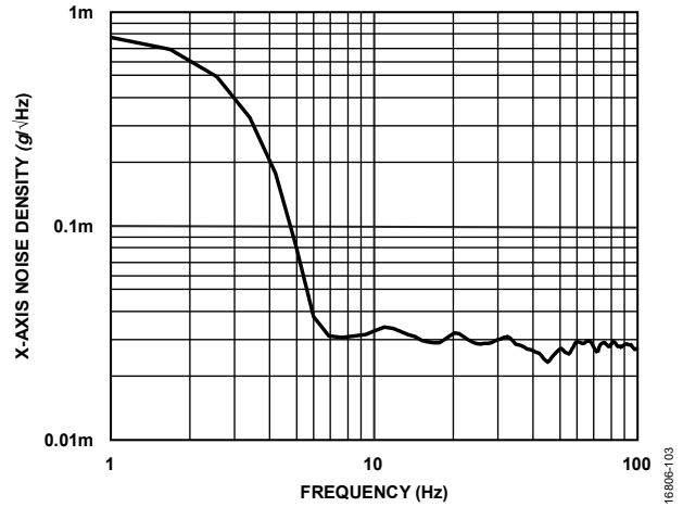
Figure 16. X-Axis Noise Density, Low Frequency, RTS Mode
