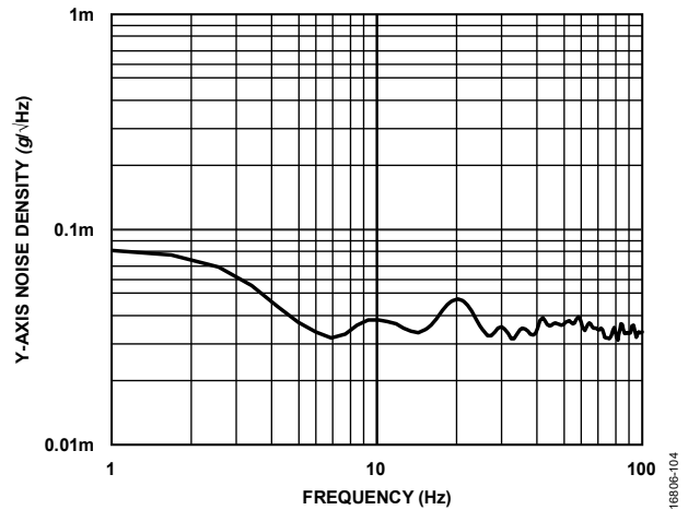
Figure 17. Y-Axis Noise Density, Low Frequency, RTS Mode
