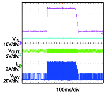
Load Dump V_{IN} = 12V \rightarrow 36V , I_{OUT} = 3A
