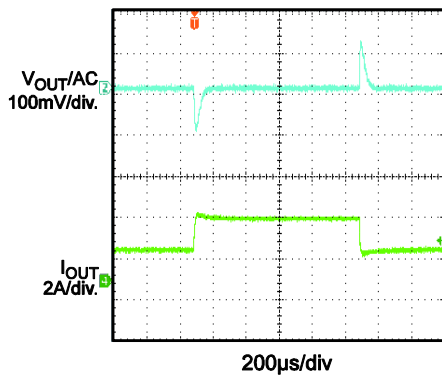
Load Transient I_{OUT} = 1.5A \rightarrow 3A , 1.6A/µs
