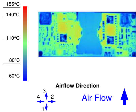
Figure 8. Thermal Image for Airflow Direction 3 (5A output, 55°C ambient, 200 LFM, typical Vin, open frame, socket interface)
