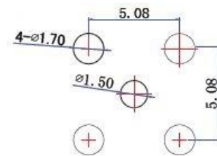
PCB Mounting Hole Pattern
