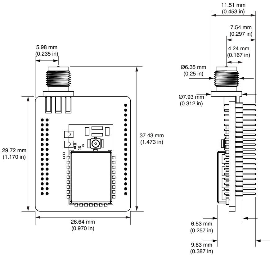
Figure 13: EVM-fff-PRC-CAS Dimensions
