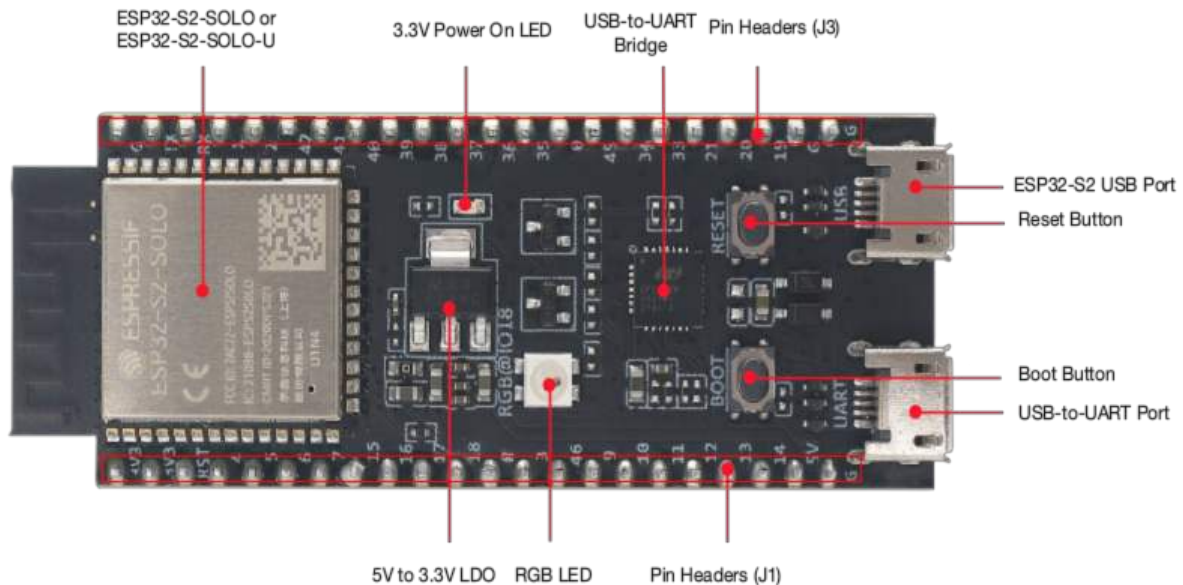
ESP32-S2-DevKitC-1 - front
