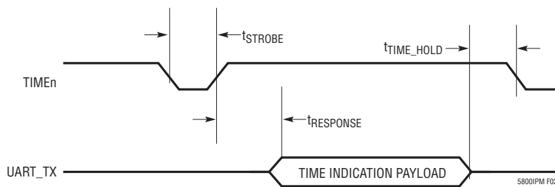
Figure 2. Timestamp Timing
