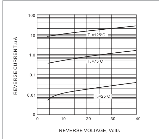
FIG. 2-TYPICAL REVERSE CHARACTERISTICS
