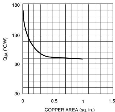
Figure 22. \theta_{JA} vs Copper (1 ounce) Area for SO PowerPAD Package
