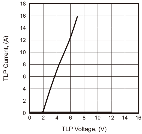
Fig.1 - Positive Clamping Voltage (TLP)
