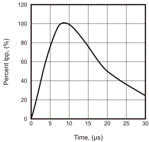
Fig.3 - IEC 61000-4-5 Test Waveform
