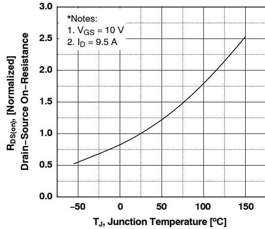
Figure 8. On-Resistance Variant vs. Temperature
