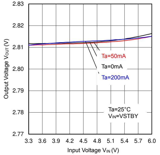
Figure 25. Line Regulation
