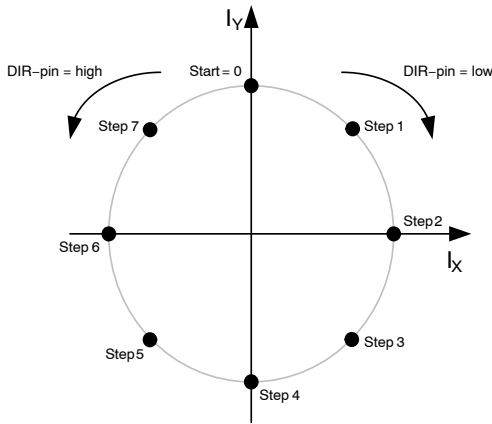
Figure 12. Half-step
