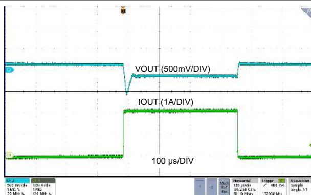
Figure 6-7. Load Transient 12 V IN , 5 V OUT , I OUT = 0 A to 2 A, Slew Rate = 1 A/μs (AUTO) with 3 × 22 μF C OUT
