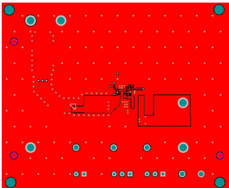
Figure 4-2. EVM Top Copper Layer
