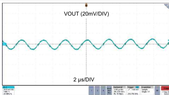
Figure 6-9. Output Ripple at 12 V IN , 5 V OUT (Fixed), 2-A Load with 2 × 22 μF C OUT
