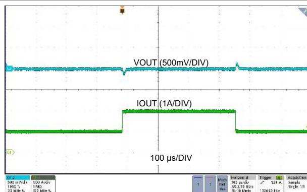
Figure 6-8. Load Transient 12 V IN , 5 V OUT , I OUT = 1 A to 2 A, Slew Rate = 1 A/μs (AUTO) with 3 × 22 μF C OUT
