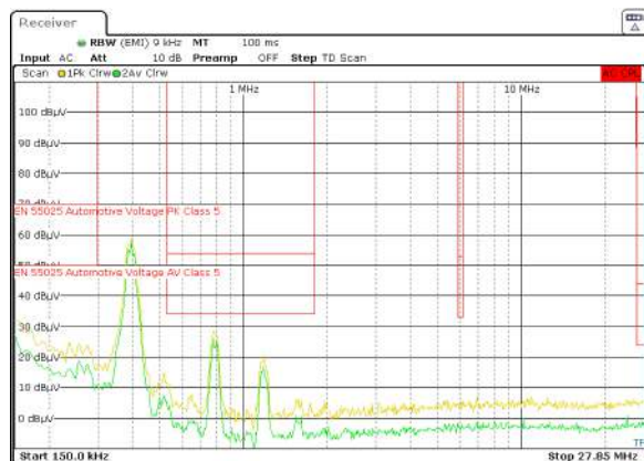
Figure 6-12. LMR43620RQ5EVM-400 Low Frequency Conducted EMI Results 12.5 V IN , 5 V OUT , I OUT = 2 A (Green-Average Scan and Yellow-Peak Scan)
