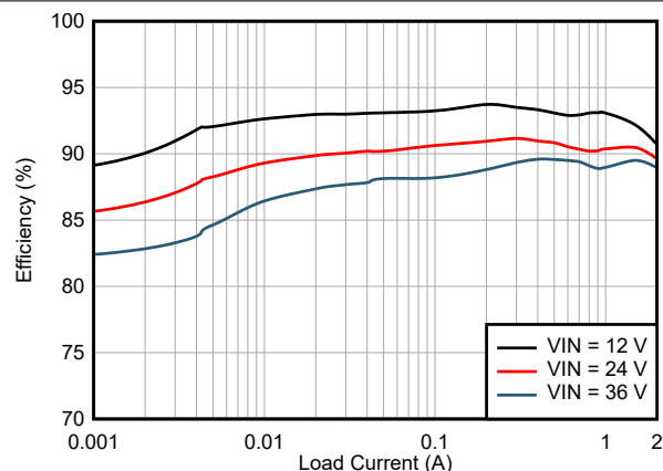
Figure 6-1. 5 V OUT , 400-kHz Efficiency
