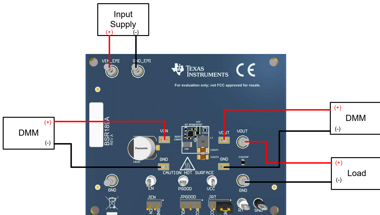
Figure 1-1. EVM Board Connections
