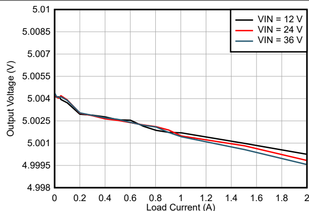
Figure 6-2. 5 V OUT , 400-kHz Load Regulation
