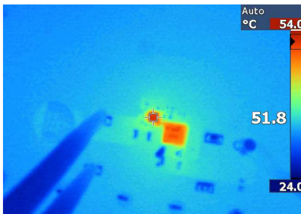
Figure 6-11. Thermal Capture, 12 V IN , 5 V OUT , 2-A Load, 400 kHz, \Theta_{JA} \approx 42^\circ\text{C/W}
