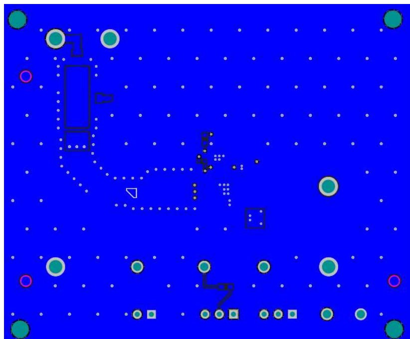
Figure 4-5. EVM Bottom Copper Layer
