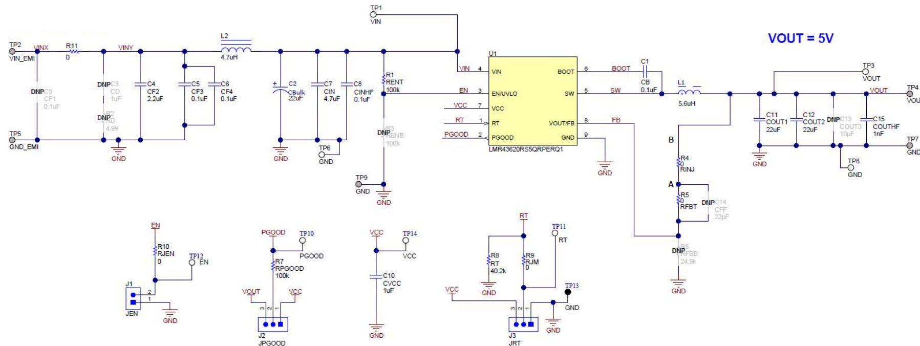
Figure 3-1. LMR43620RQ5EVM-400 Schematic
