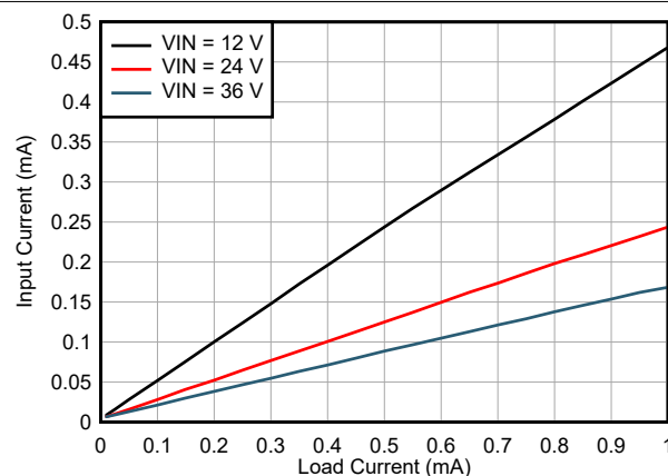
Figure 6-4. Input Current vs Load Current for 5 V OUT
