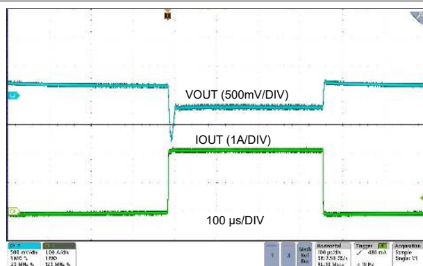
Figure 6-5. Load Transient 12 V IN , 5 V OUT , I OUT = 0 A to 2 A, Slew Rate = 1 A/μs (AUTO) with 2 × 22 μF C OUT
