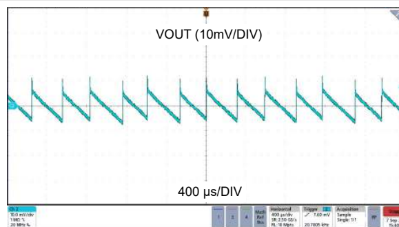
Figure 6-10. Output Ripple at 12 V IN , 5 V OUT (Fixed), 1 mA Load with 2 × 22 μF C OUT
