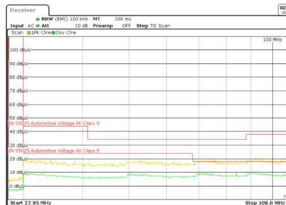
Figure 6-13. LMR43620RQ5EVM-400 High Frequency Conducted EMI Results 12.5 V IN , 5 V OUT , I OUT = 2 A (Green-Average Scan and Yellow-Peak Scan)
