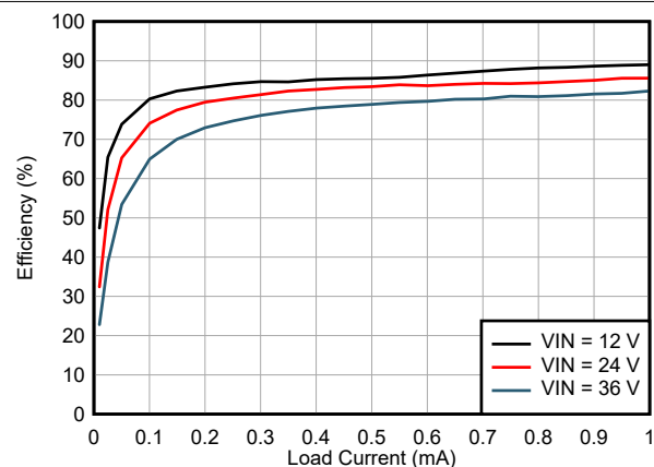
Figure 6-3. 5 V OUT , Light Load Efficiency
