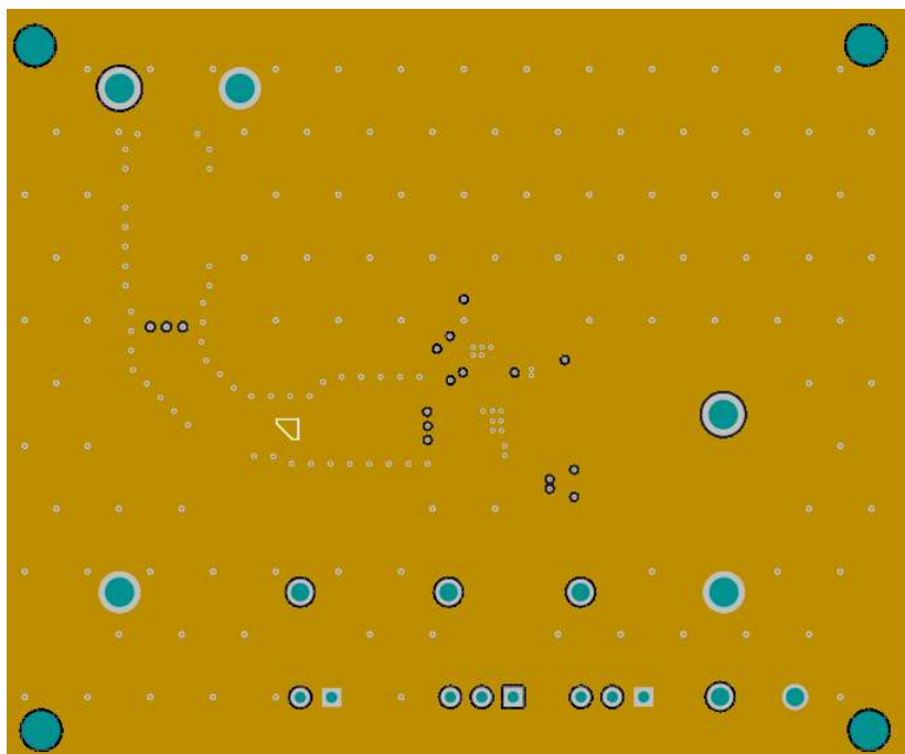
Figure 4-3. Mid-Layer One
