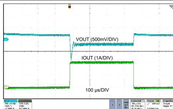
Figure 6-6. Load Transient 24 V IN , 5 V OUT , I OUT = 0 A to 2 A, Slew Rate = 1 A/μs (AUTO) with 2 × 22 μF C OUT
