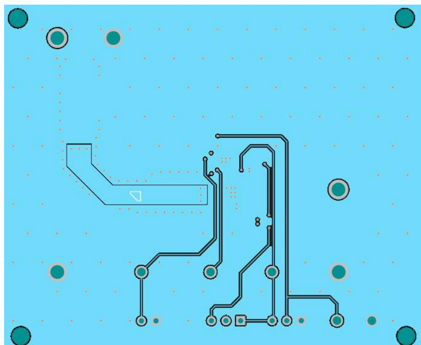
Figure 4-4. Mid-Layer Two
