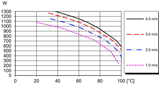
Available output power vs. ambient air temperature and airflow. See Thermal Consideration section.
