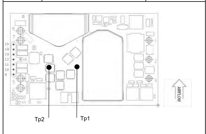
Base plate (Bottom view)
