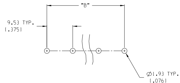
PTH PATTERN
