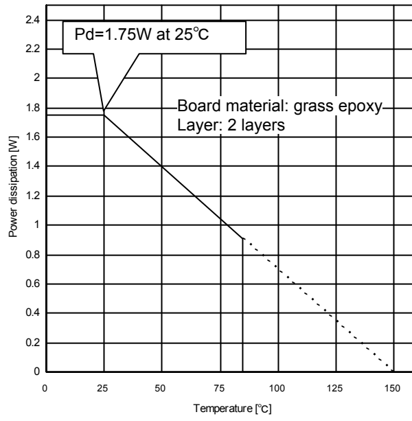
Figure 25. Power Dissipation [W] vs. Temperature [°C]
