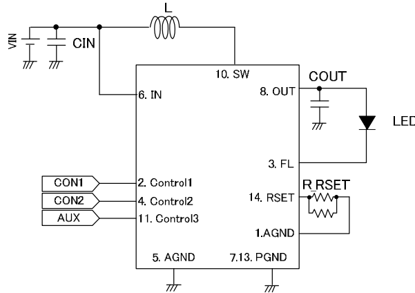
Figure 23. Application Circuit
