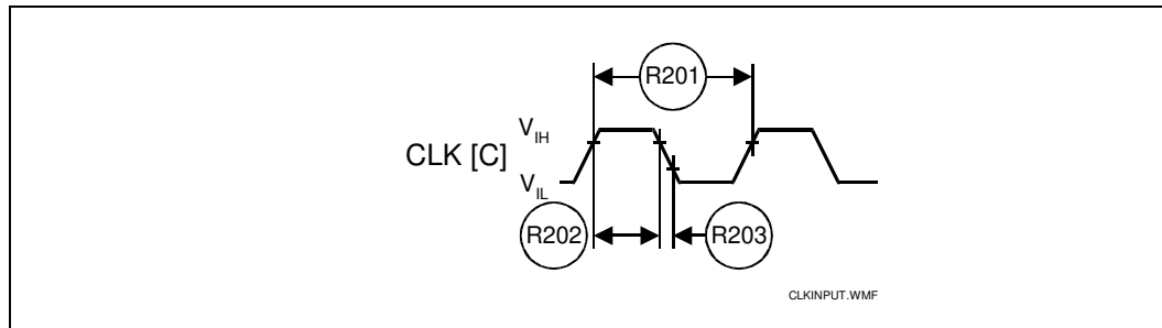
Figure 13. Clock Input AC Waveform
