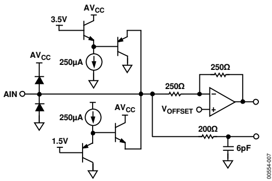
Figure 20. Analog Input Stage
