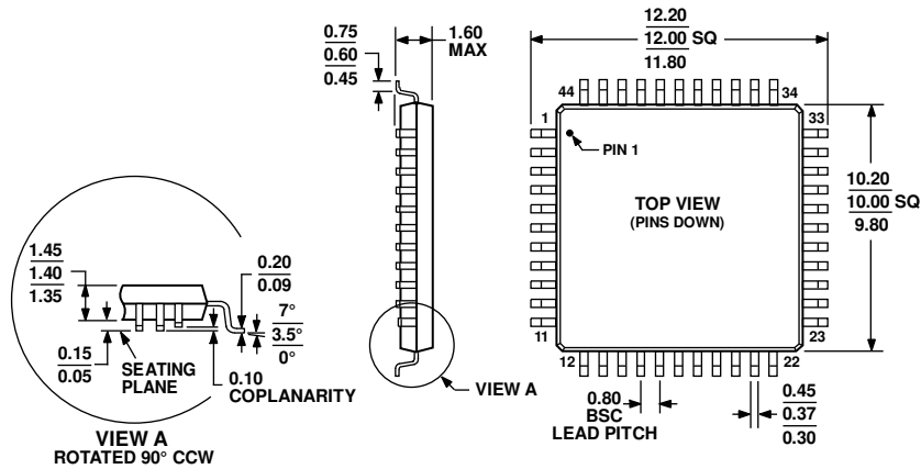
Figure 46. 44-Lead Low Profile Quad Flat Package [LQFP] (ST-44-1)
