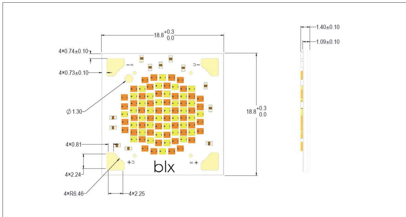
Figure 12: Drawing for Vesta Series Tunable White 13mm Array
