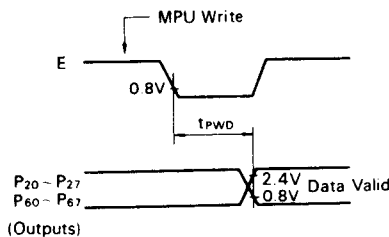
Figure 6 Port Data Delay Times (MPU Write)
