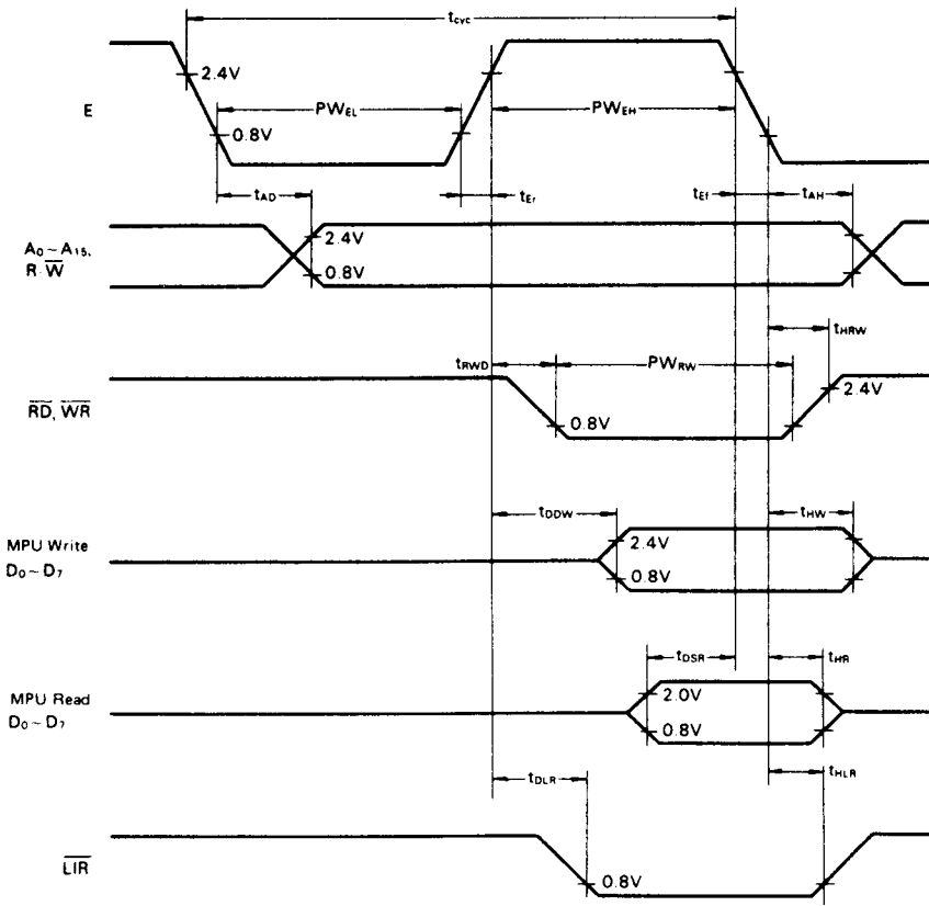
Figure 1 Bus Timing
