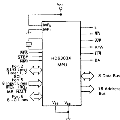
Figure 15 Operation Mode
