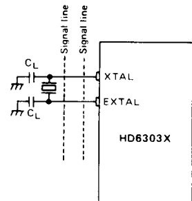
Figure 26 Warning concerning board design of oscillation circuit
