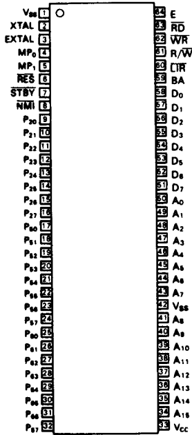
(Top View)
