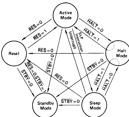
Figure 24 CPU Operation Mode Transition
