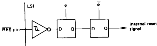
Figure 30 \overline{\text{RES}} circuit
