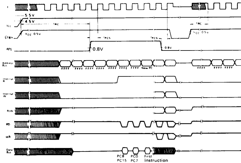
Figure 11 Reset Timing
