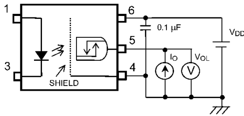
Fig. 12.1.1 V_{OL} Test Circuit
