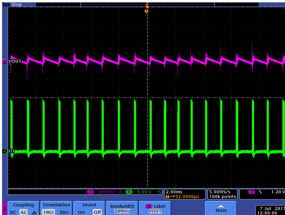
Figure 11. Burst Mode at V_{in} = 390\text{-V} and 100-mA Load (Ch3 = V_{out} ; Ch4 = LO)
