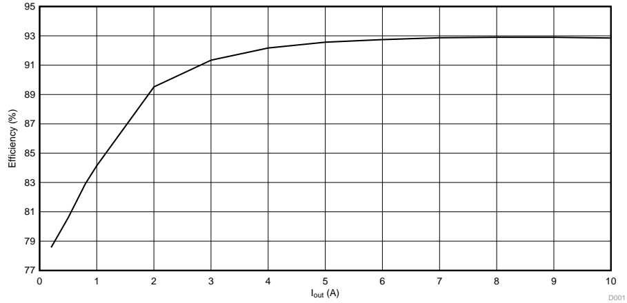
Figure 4. UCC25630-1EVM-291 Efficiency
