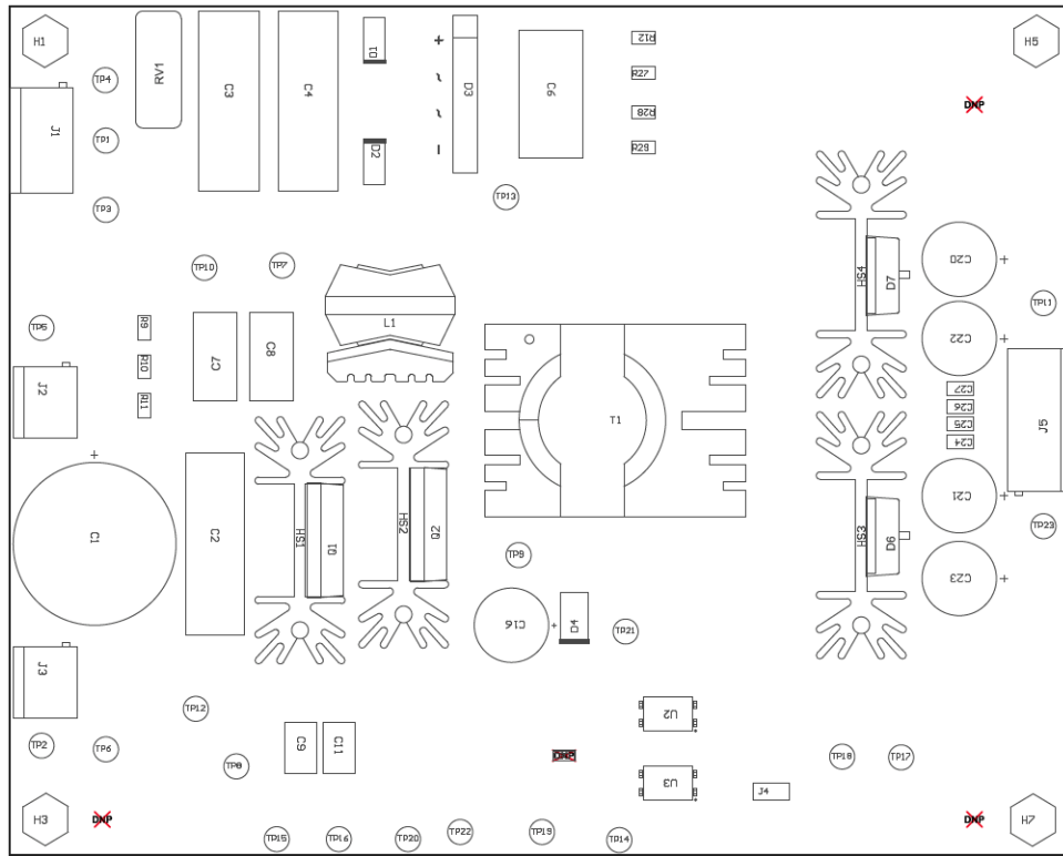
Figure 16. UCC25630-1EVM-291 Top Layer Assembly Drawing (Top View)
