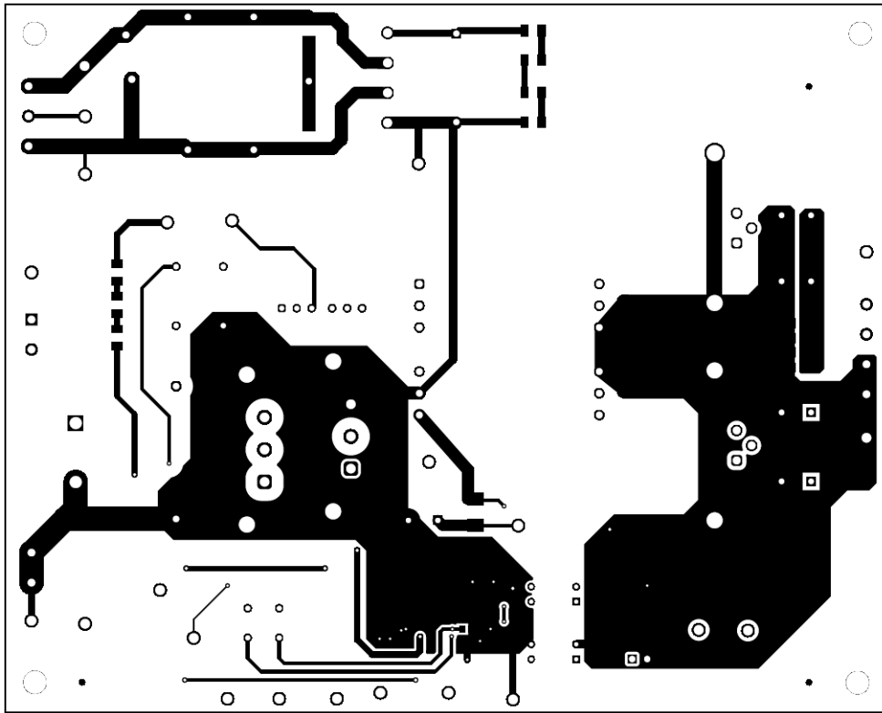
Figure 18. UCC25630-1EVM-291 Top Copper (Top View)
