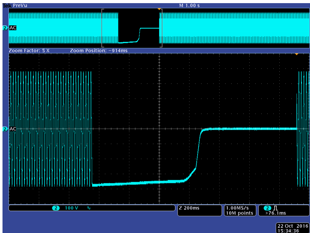
Figure 13. X-Cap Discharge
