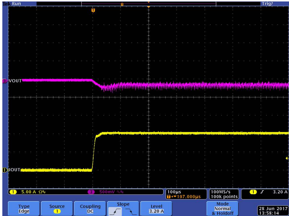
Figure 8. No Load (0 A) to Full Load (10 A) Transient (Ch1 = I out ; Ch3 = V out )
