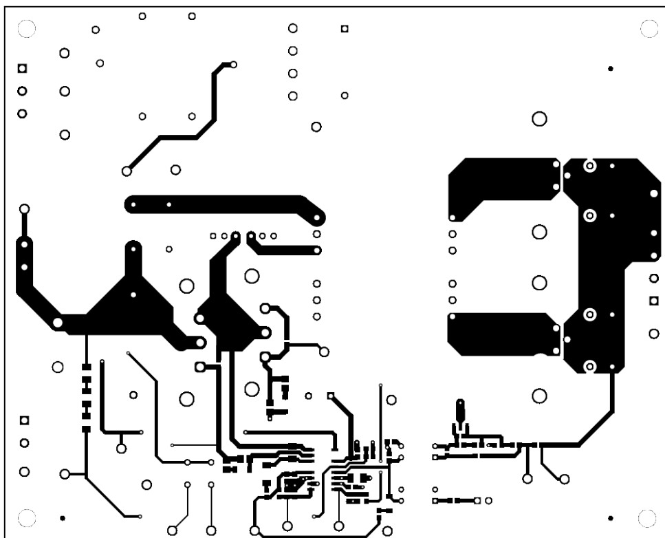
Figure 19. UCC25630-1EVM-291 Bottom Copper (Top View)
