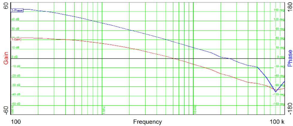
Figure 14. Bode Plot at V_{in} = 390 V and 10 A Load
