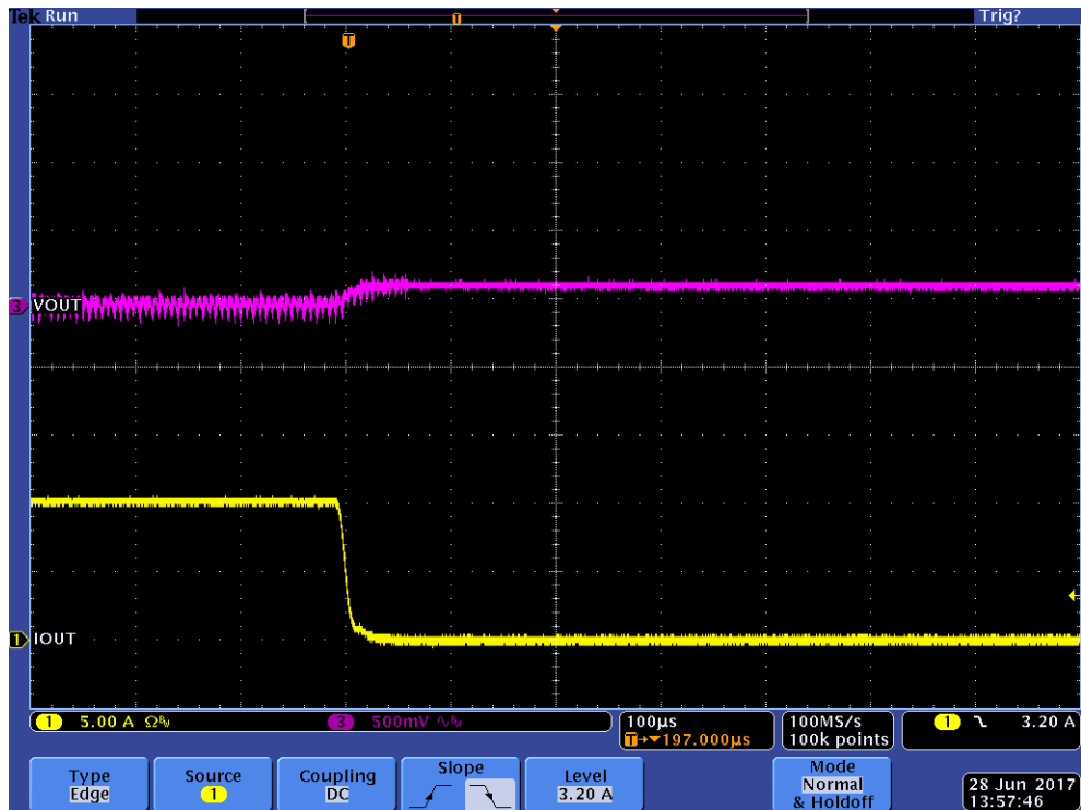
Figure 9. Full Load (10 A) to No Load (0 A) Transient (Ch1 = I out ; Ch3 = V out )
