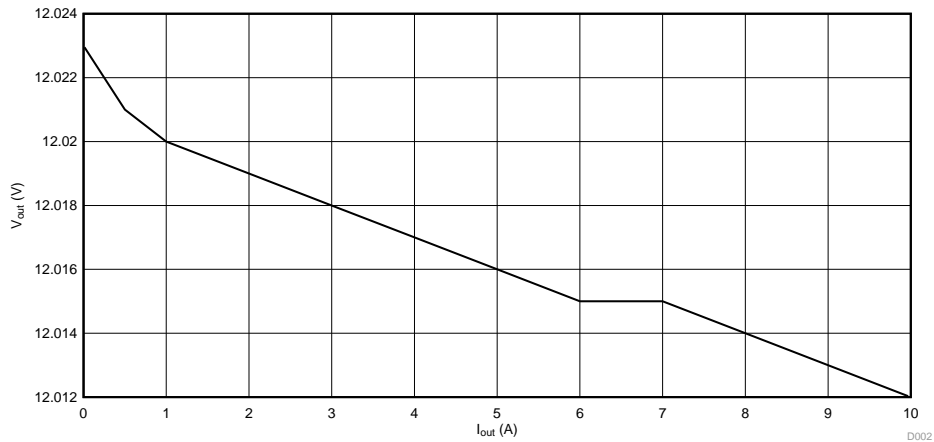
Figure 5. UCC25630-1EVM-291 Load Regulation
