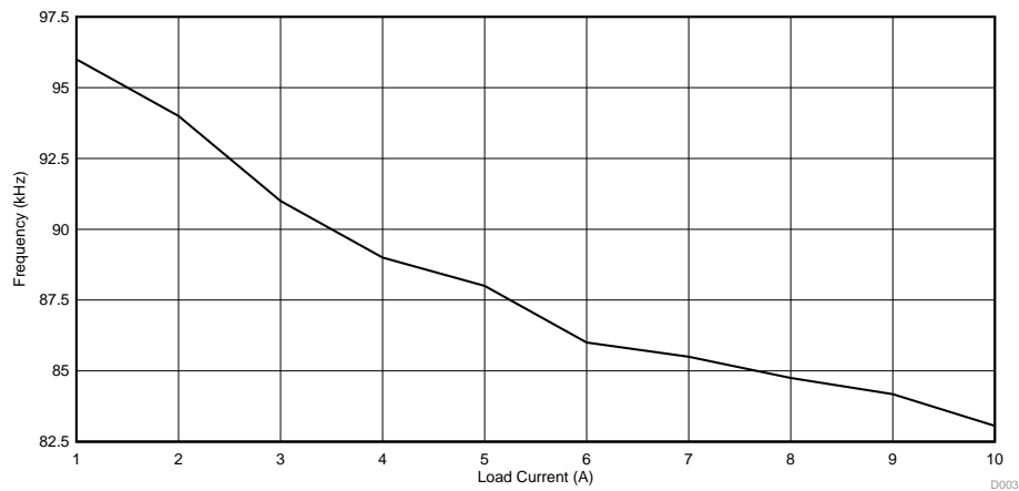
Figure 15. Switching Frequency vs. Load ( V_{in} = 390 V )
