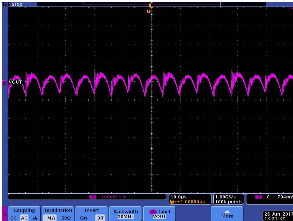
Figure 10. Output Voltage Ripple at V_{in} = 390\text{-V} and 10-A Load
