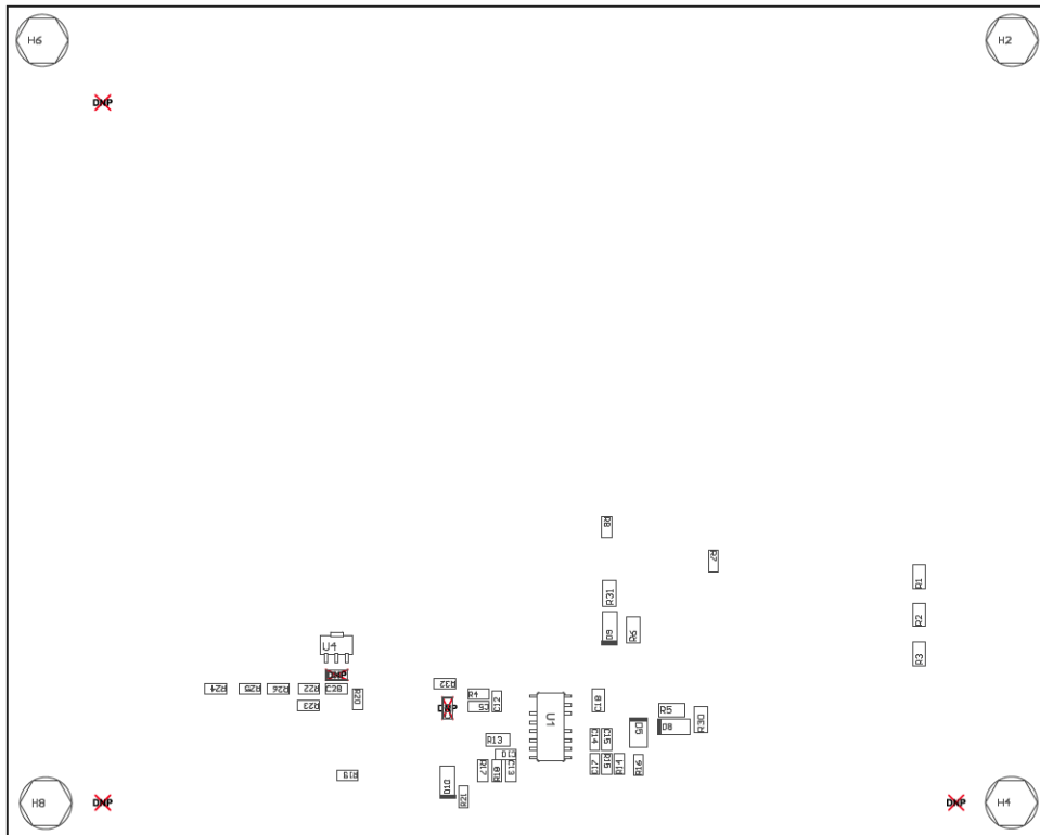
Figure 17. UCC25630-1EVM-291 Bottom Layer Assembly Drawing (Bottom View)
