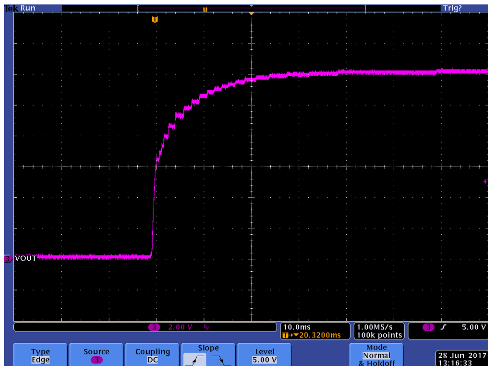
Figure 7. Output Turn On at 390 VDC with No Load
