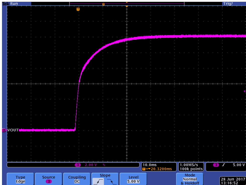
Figure 6. Output Turn On at 390 VDC with Full Load (10 A)
