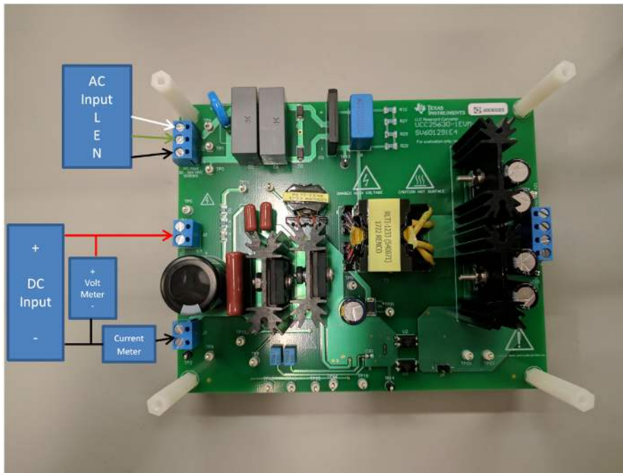
Figure 2. UCC25630-1EVM-291 Recommended Test Setup for No Load
