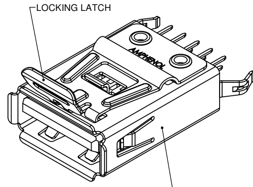
TYPE A USB 3.0 RECEPTACLE
