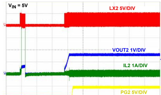
FIGURE 30. OUTPUT SHORT CIRCUIT RECOVERY (FROM HICCUP) CHANNEL 2
