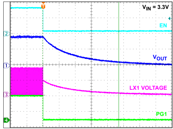
FIGURE 43. SOFT-DISCHARGE SHUTDOWN
