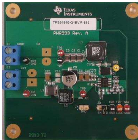
Figure 1. TPS54540-Q1EVM-593 Board
