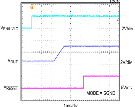
SOFT-START WITH 2.5V PREBIAS, 5V OUTPUT, PWM MODE, FIGURE 4A CIRCUIT TOC16
