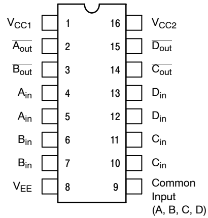
Figure 2. Pin Assignment
