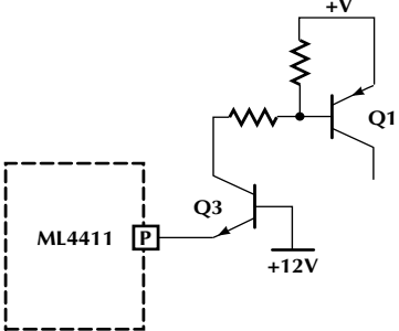
Figure 18. High Voltage Translation using PNP Power Transistor
