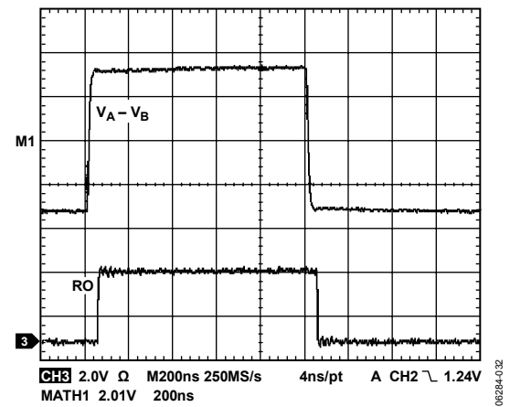
Figure 27. ADM3490E/ADM3491E Receiver Propagation Delay, Driven by External RS-485 Device
