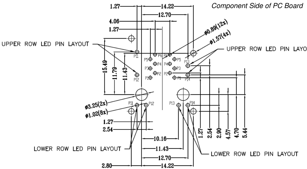
Figure 18: 6 Position Jack, 2x1p with LED
