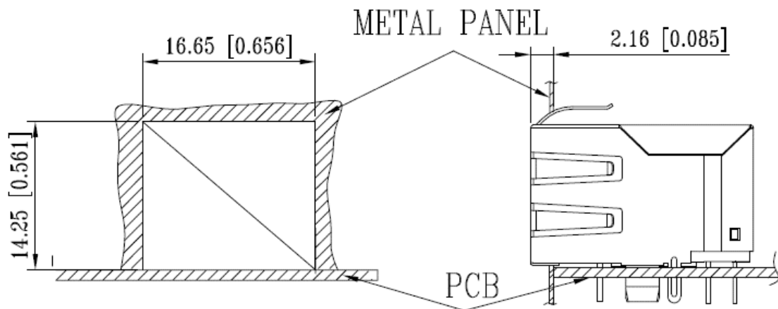
Figure 35: 10 position Jack with and without LED, Tab down (2301994-6 / 2301994-7 / 1-2301994-0 / 1-2301994-2 / 2-2301994-1 / 2-2301994-2 / 2-2301994-3 / 2-2301994-4)
