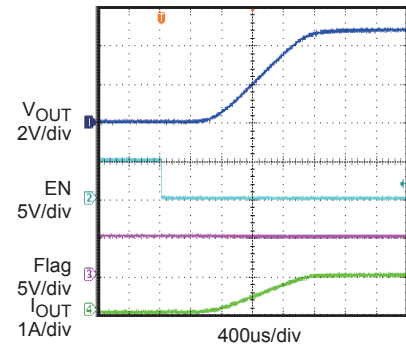
Turn On Delay and Rise Time with 100μF Load I_{OUT}=1A , C_L=100\mu F
