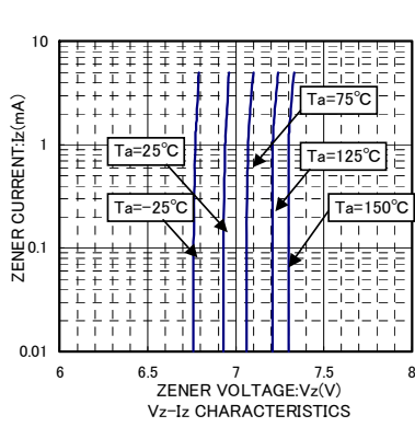
V_z - I_z CHARACTERISTICS
