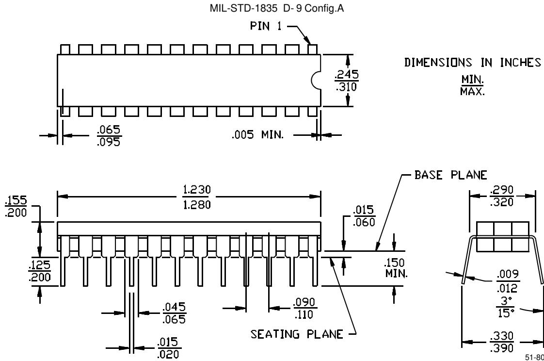
Figure 3. 24-Lead (300-Mil) PDIP P13
