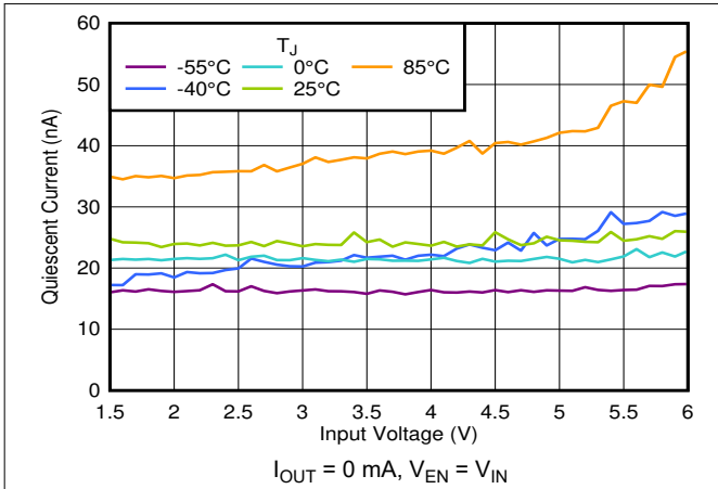
Figure 6-1. I_Q vs V_{IN} and Temperature
