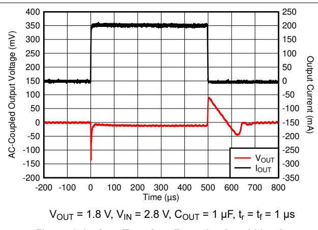
Figure 6-14. I_{OUT} Transient From 1 mA to 200 mA
