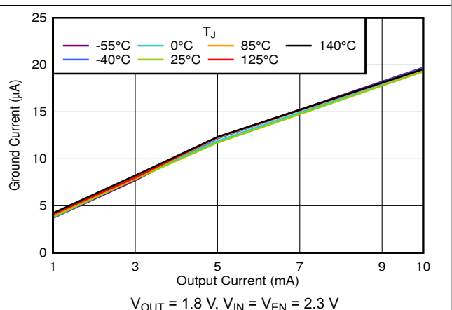
Figure 6-6. I_Q vs I_{OUT} and Temperature for 1 mA to 10 mA
