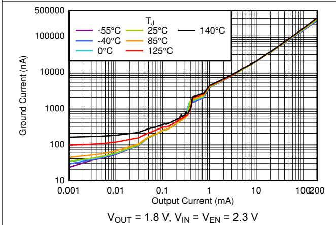
Figure 6-3. I_Q vs I_{OUT} and Temperature up to 200 mA
