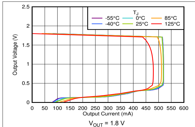
Figure 6-37. Foldback Current Limit vs I_{OUT} and Temperature
