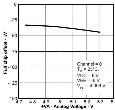
Figure 32. Full Chip Offset Error vs Analog Supply Voltage (+VA)
