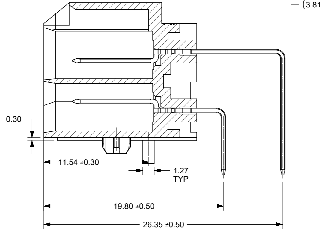
SECTION B-B
