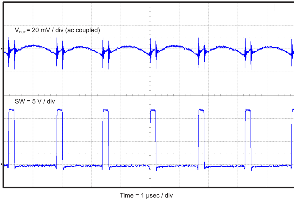
Figure 4-6. TPS56428EVM-534 Output Voltage Ripple ( I_{OUT} = 4 A)
