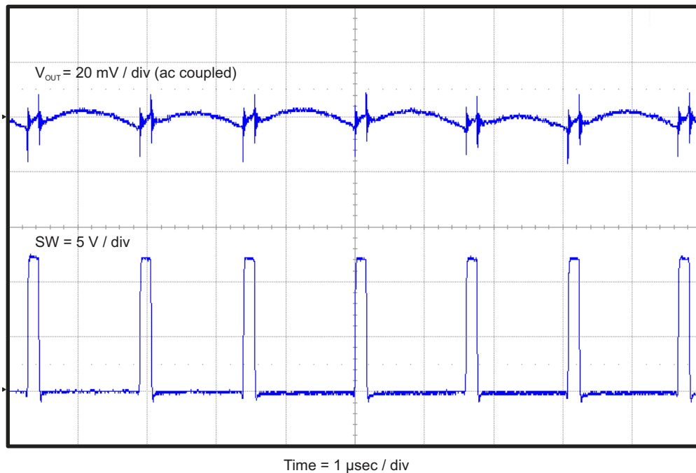
Figure 4-7. TPS56428EVM-534 Output Voltage Ripple ( I_{OUT} = 500 mA)
