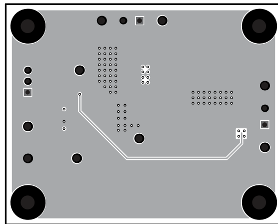
Figure 5-5. Bottom Layer
