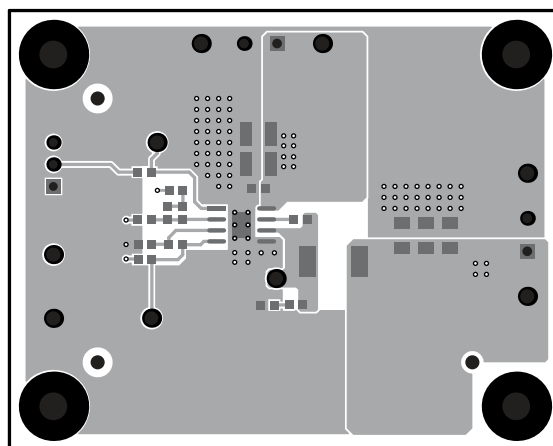
Figure 5-2. Top Layer
